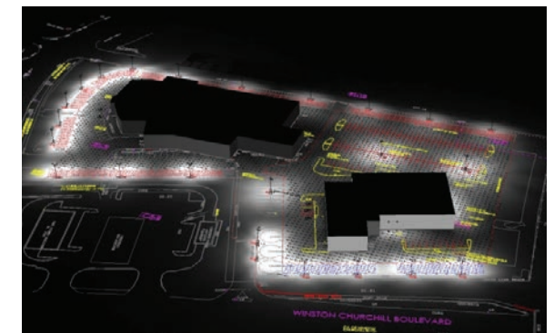
Technical Design and Renderings
